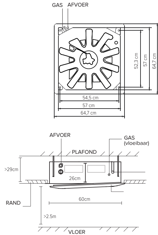
9 - 18K ceiling hole size
