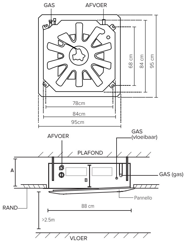
24 - 48K ceiling hole size
